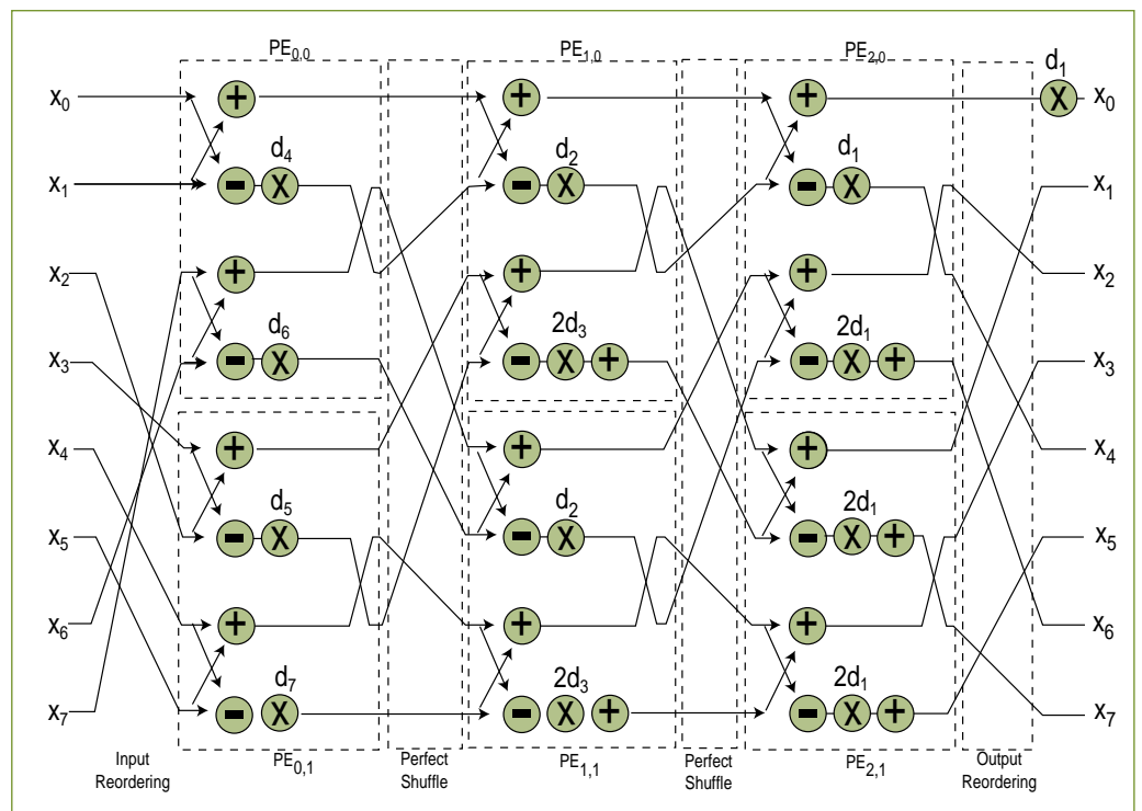
Figure 1 DCT8x8 Algorithm
