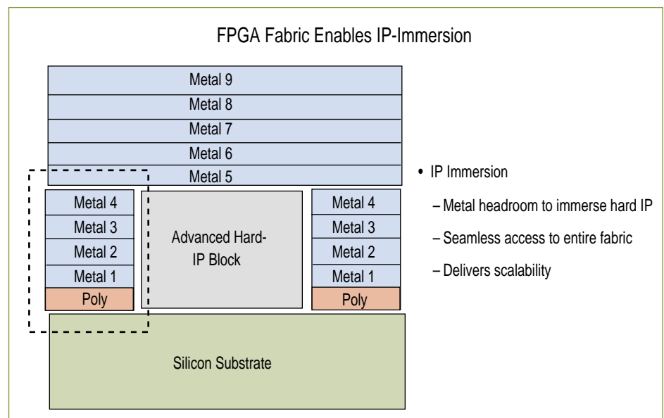
Figure 1 Hard IP-immersion embeds low- and medium-complexity hard IP blocks into FPGAs, such as Block RAM and multipliers. The cross section of the silicon die shows metal headroom over the immersed hard IP block. By contrast, Soft IP-immersion enables users to integrate soft IP into any location of the FPGA and move it around without any performance or access penalties.
