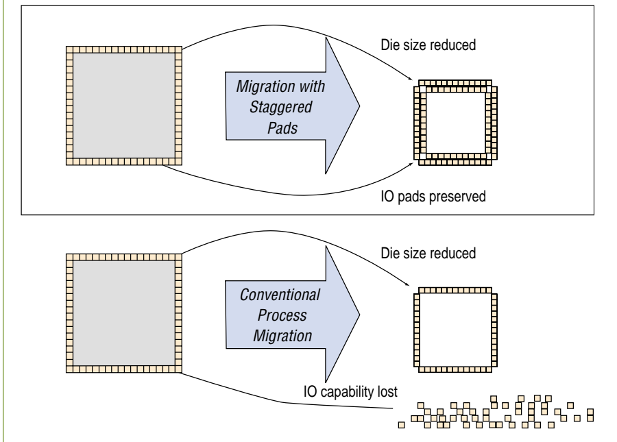
Figure 2 Staggered Pad Technology allows reduction in die size while preserving the number of I/O pads.
