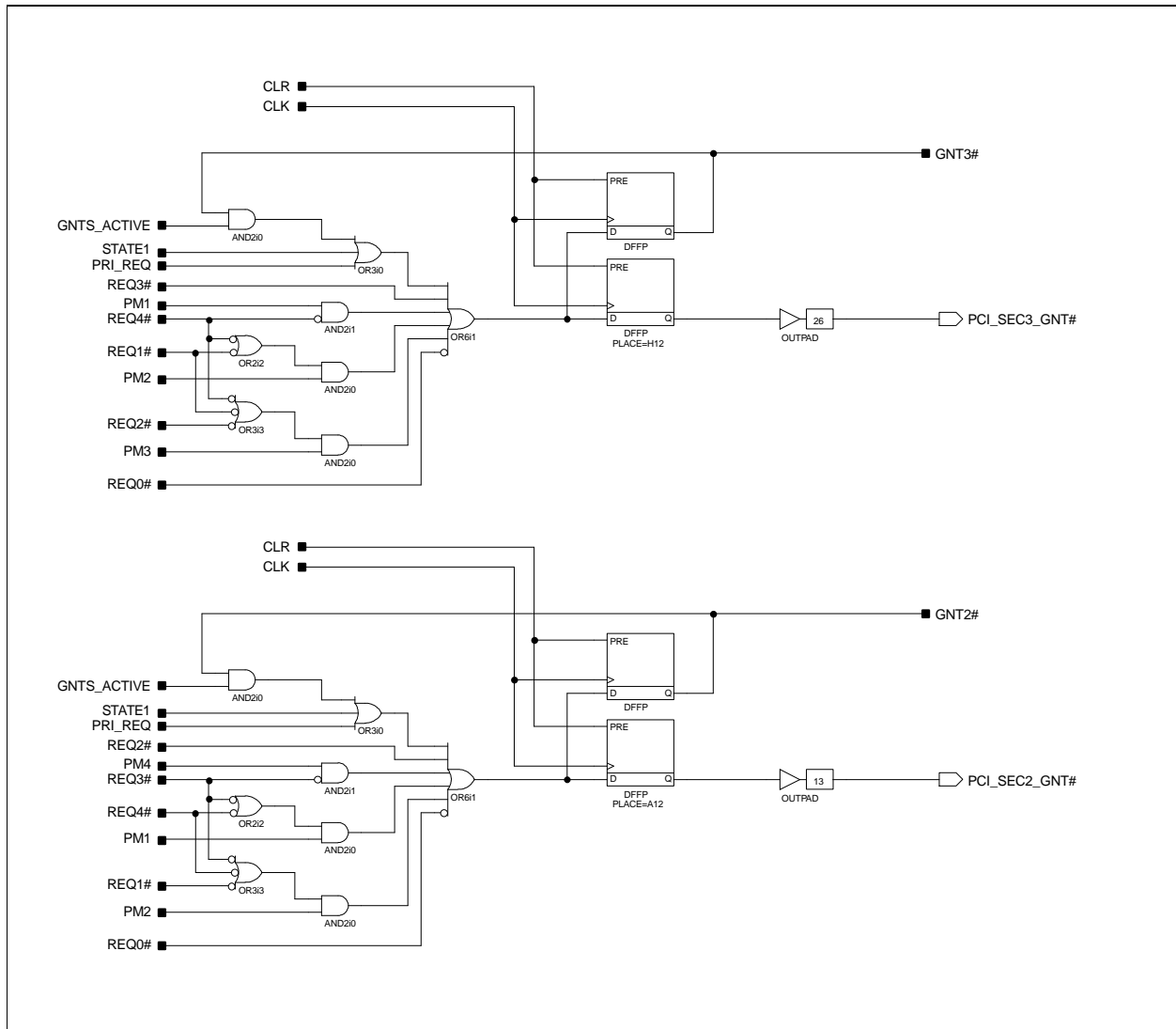
PCI Arbiter FPGA—Sheet 2
