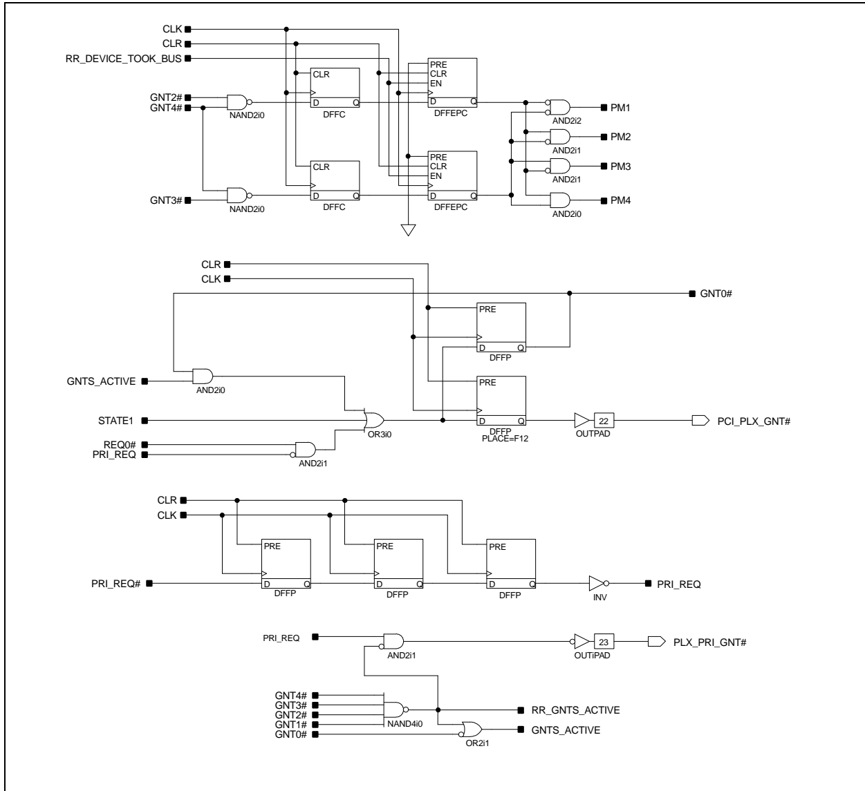
PCI Arbiter FPGA—Sheet 4
