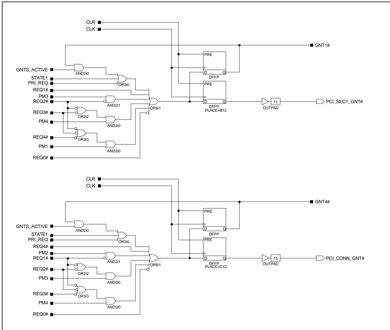
PCI Arbiter FPGA—Sheet 3
