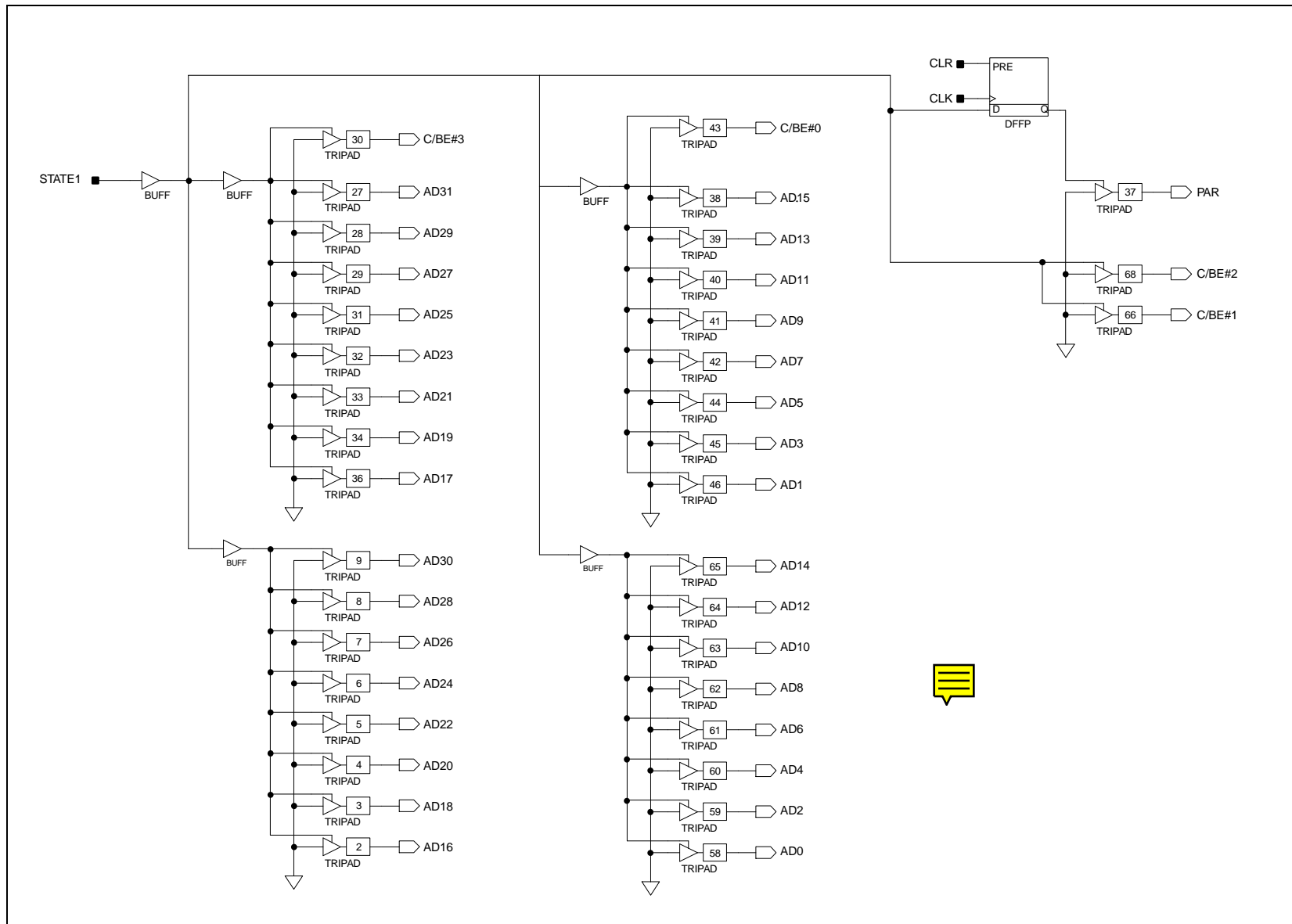
PCI Arbiter FPGA—Sheet 5
