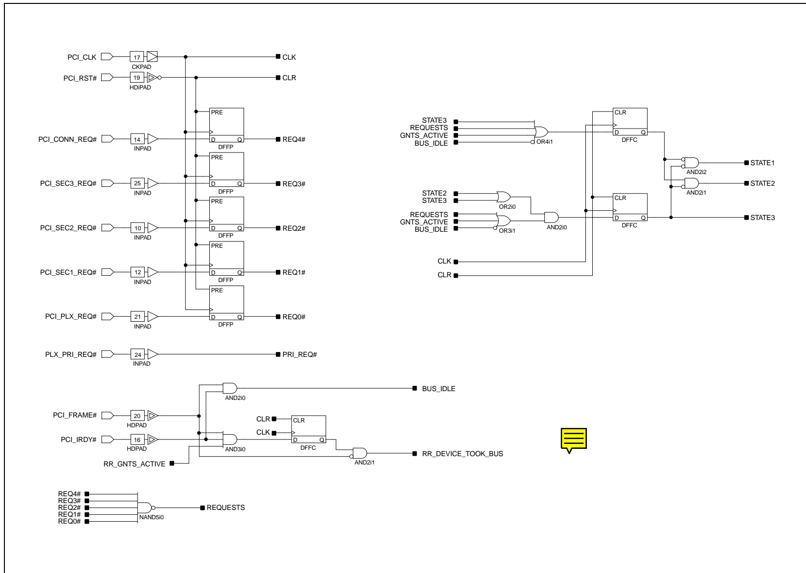
PCI Arbiter FPGA—Sheet 1
